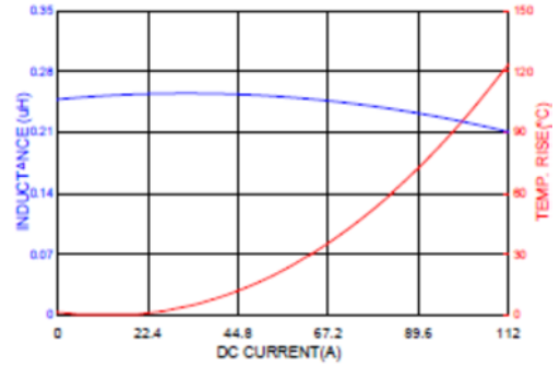
HMPL1265HP-R22
