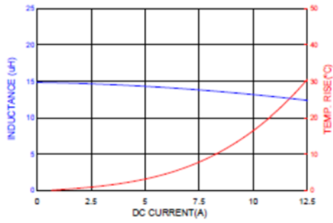
HMPL1265HP-150
