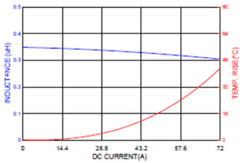
HMPL1265HP-R30
