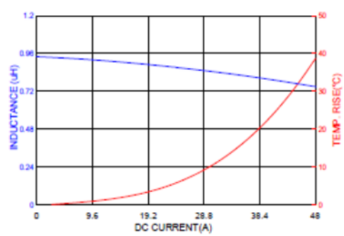
HMPL1265HP-1R0
