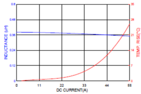
HMPL1265HP-R68
