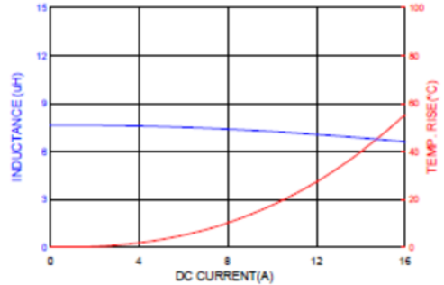
HMPL1265HP-8R2
