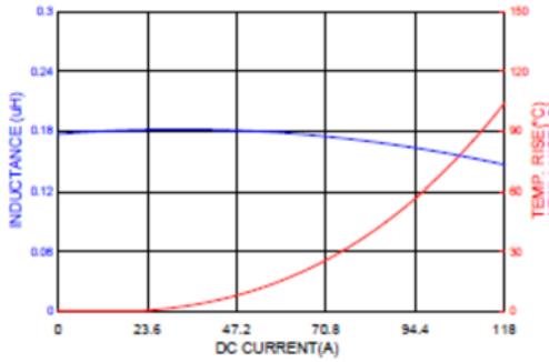
HMPL1265HP-R15
