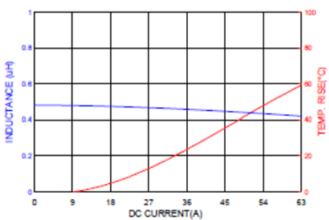
HMPL1265HP-R47
