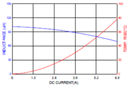
HMPL1265HP-101
