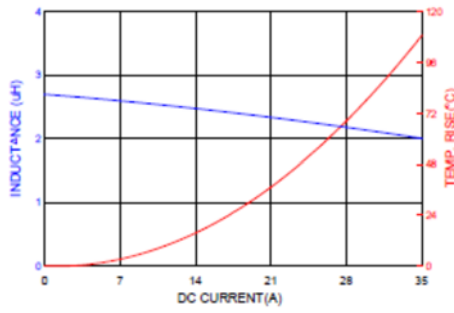
HMPL1265HP-2R7
