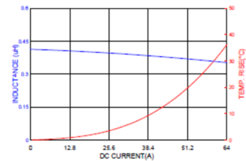
HMPL1265HP-R40
