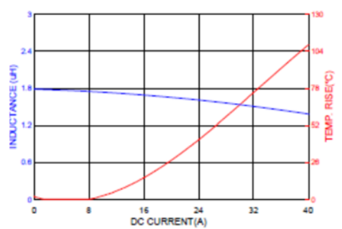
HMPL1265HP-1R8
