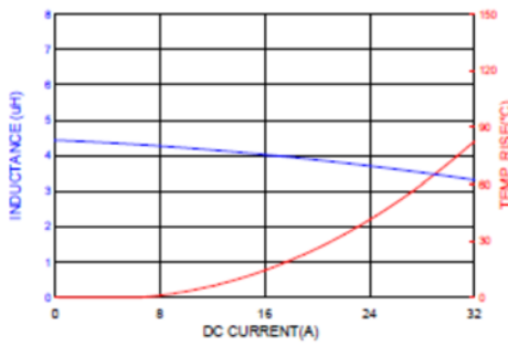
HMPL1265HP-4R7
