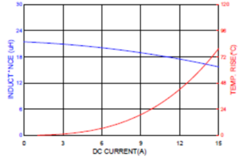
HMPL1265HP-220
