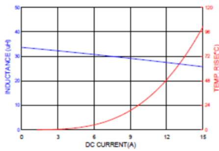
HMPL1265HP-330
