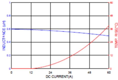
HMPL1265HP-R56
