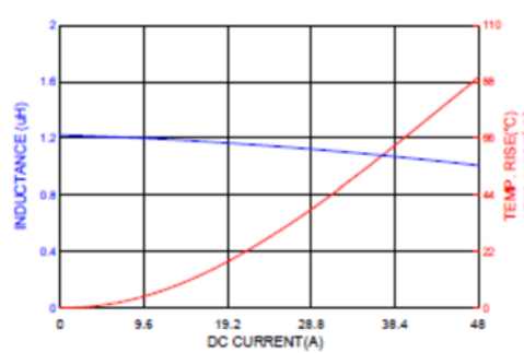
HMPL1265HP-1R2
