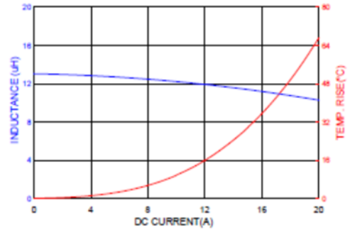
HMPL1265HP-130
